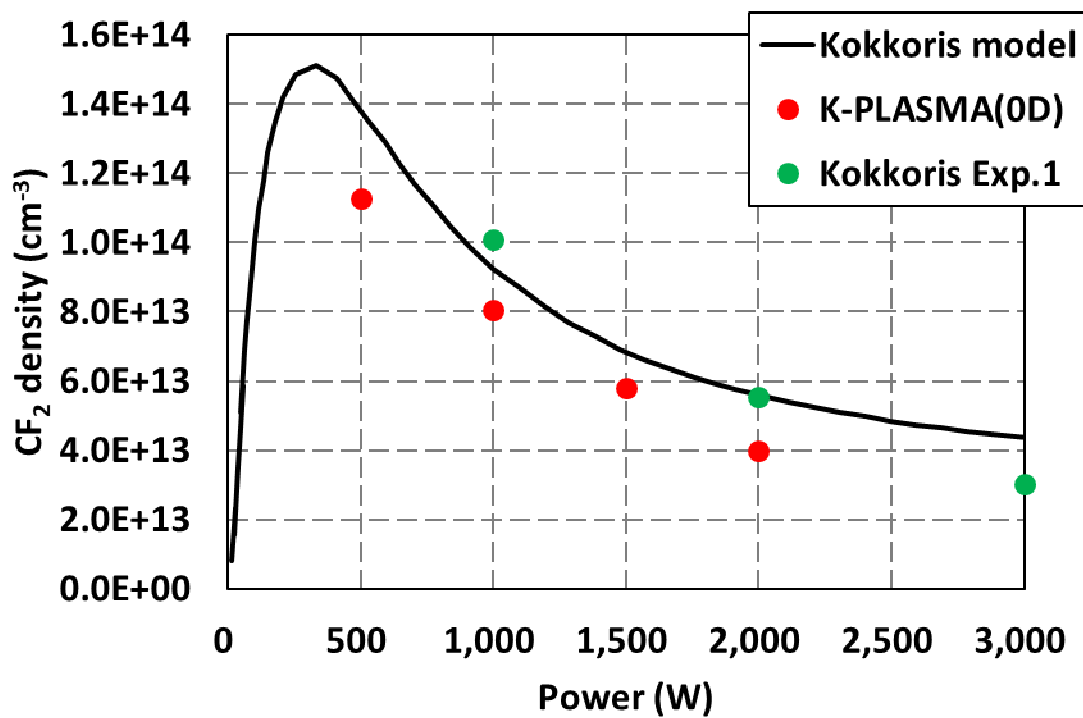
Figure 1 Comparison of CF 2 radical density as a function of source power between K-PLASMA(0D), the Kokkoris model, and the experimental data (Exp.1) reported by Kokkoris et al 1 .
