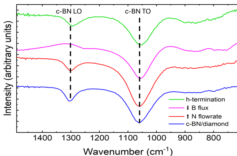
Figure 3. FTIR of c-BN growths. Illustrates variation in LO and TO mode peak areas.
