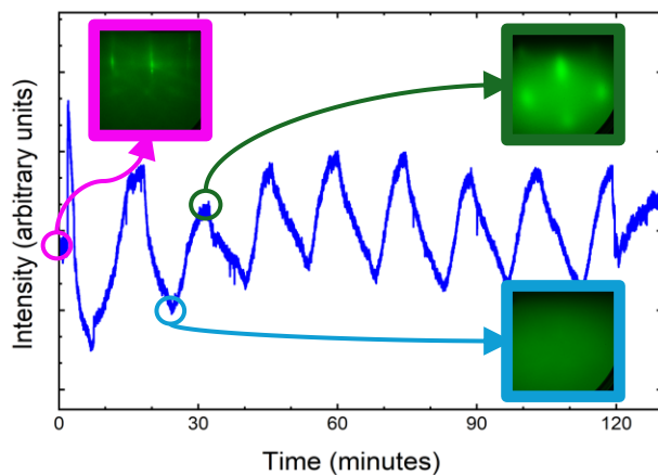
Figure 2. RHEED intensity plot over time. Purple outlined image is the substrate just before growth. Blue outlined image is blank screen at the end of each open shutter cycle (troughs). Green outlined image is the c-BN surface at the end of each closed shutter cycle (peaks).
