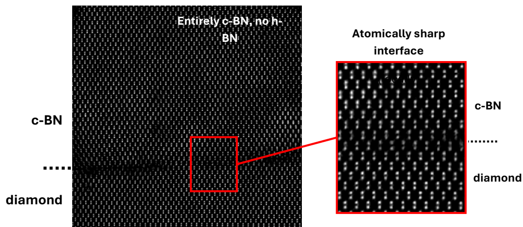
Figure 1. Electron ptychographic phase image of c-BN/Diamond interface. Inset red box shows a zoom in of the locally sharp interface.
