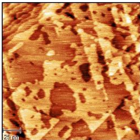
Figure 2: Ambient STM topographic image of the Au(111) surface after 5 h immersion in saturated DDQ solution in 0.1 M HClO 4 , showing changes in the Au surface morphology following exposure to DDQ
