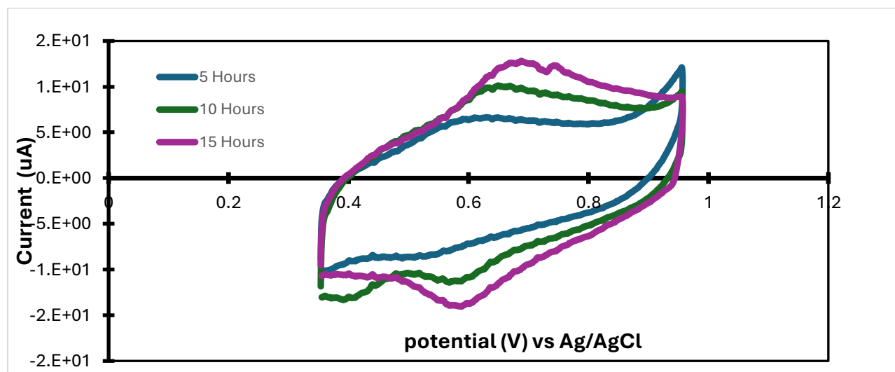
Figure 1: Cyclic voltammograms of DDQ-modified Au(111) surfaces prepared by immersion in saturated DDQ solution for different time periods.
