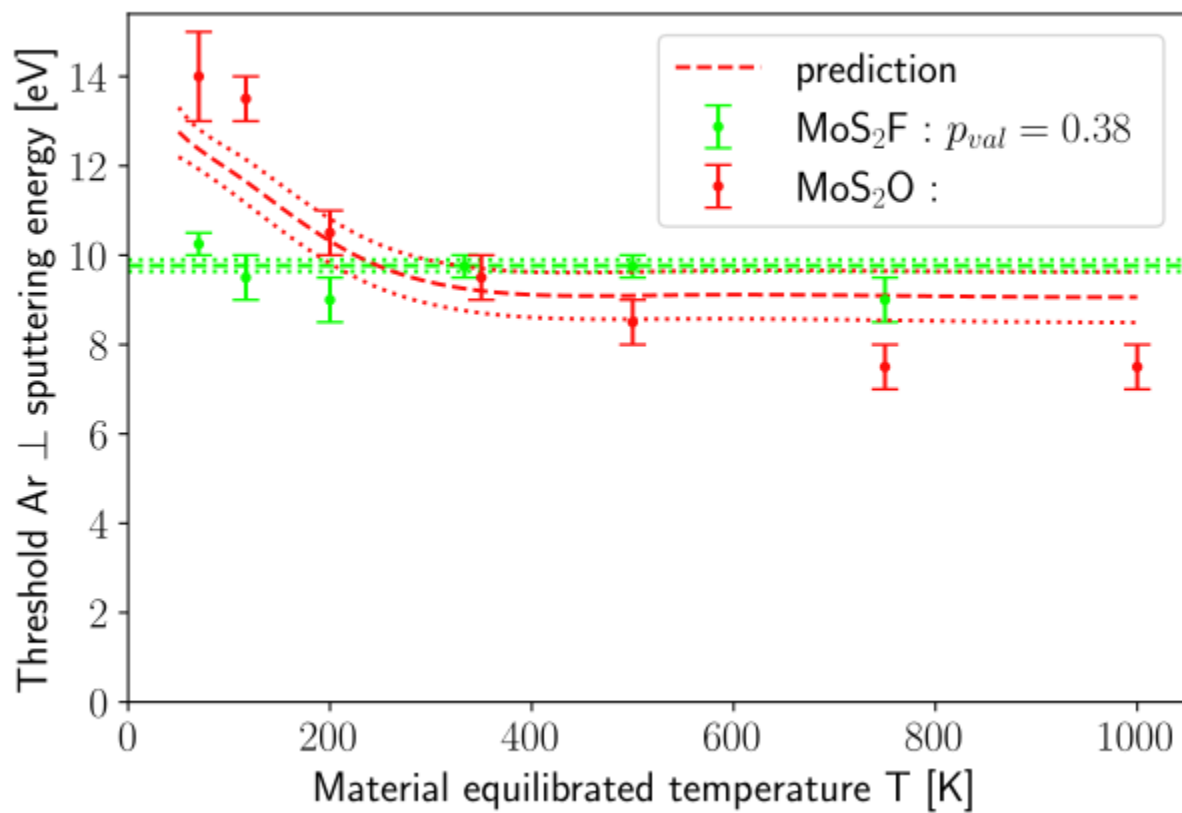
Simulated vs predicted Sulfur sputtering
