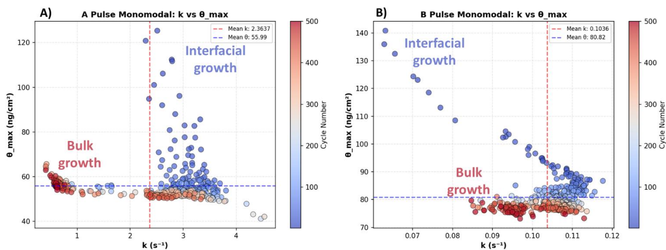
Figure 1: Scatter plot of the rate constants ( k ) and ( \theta_{\text{max}} ) surface coverage from the in-situ kinetics modelling of 500 cycles of A) Trimethyl Aluminum and B) Fumaric Acid.
