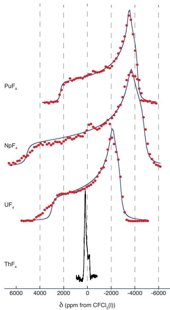
Figure 1: Room temperature ^{19}\text{F} NMR spectra of \text{AnF}_4 powders recorded in an applied field of 7.046 T.
