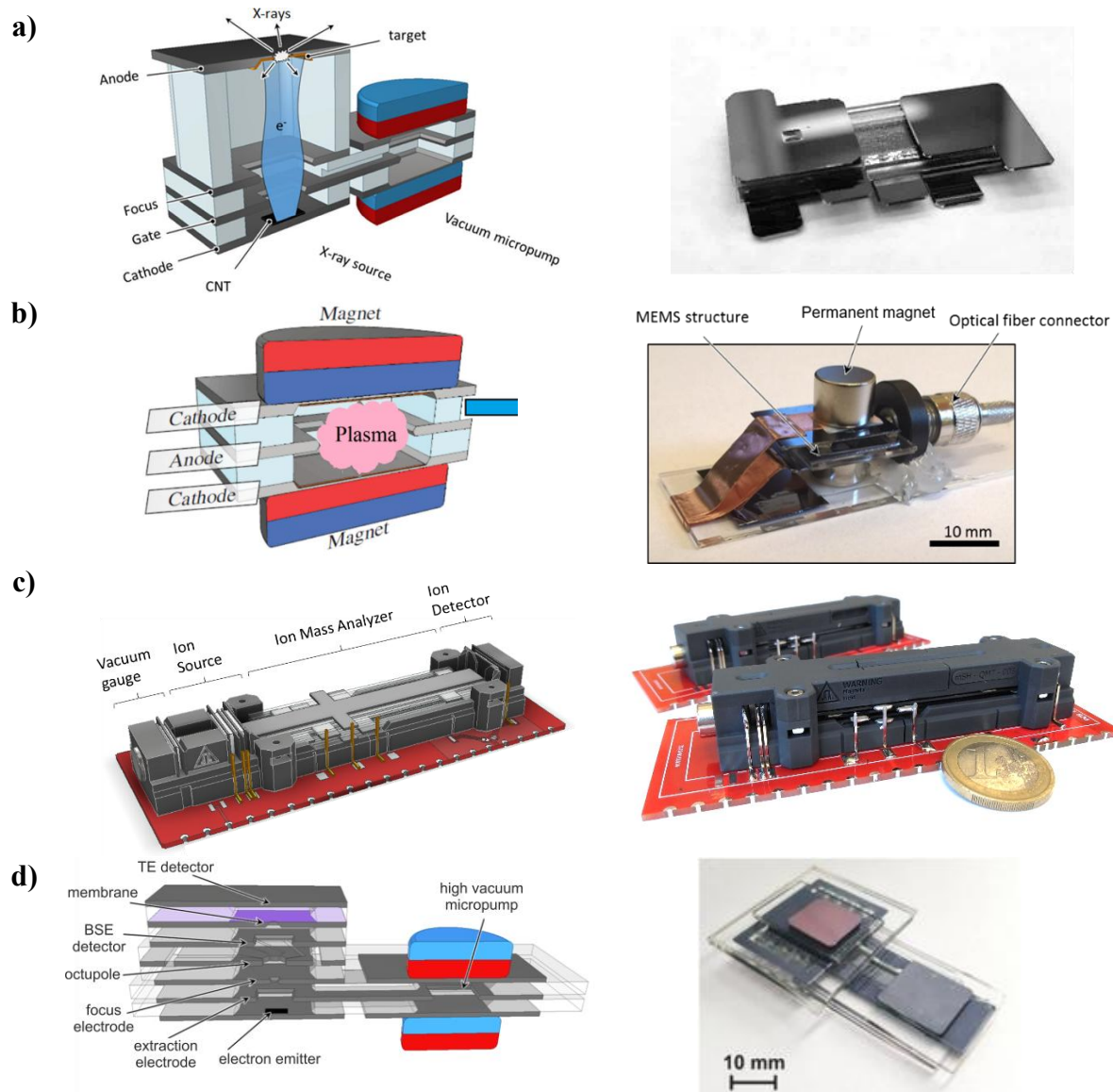
Fig. 1. Family of high vacuum MEMS analytical instruments (schematics – left column, real instruments – right column): a) MEMS X-ray source, b) MEMS plasma spectrometer, c) MEMS mass spectrometer, d) MEMS scanning electron microscope.
