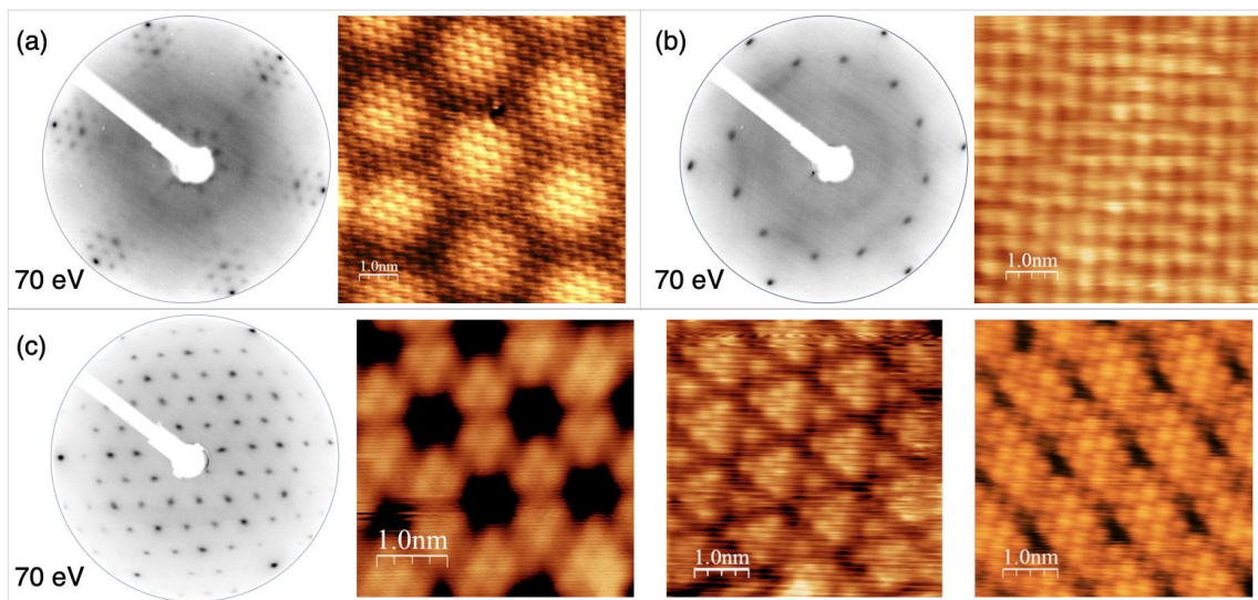
Fig. 1. LEED and STM images showing hexagonal (a), square (b), and multiple 5x5 phases (c) on Au(111).
