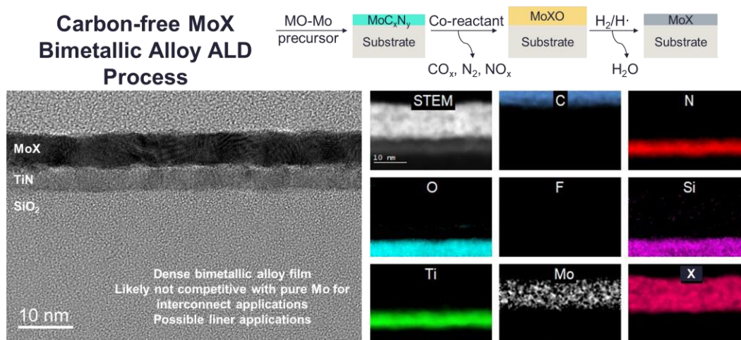
Figure 2. New ALD process for carbon-free bimetallic alloy from a MO-Mo precursor.
