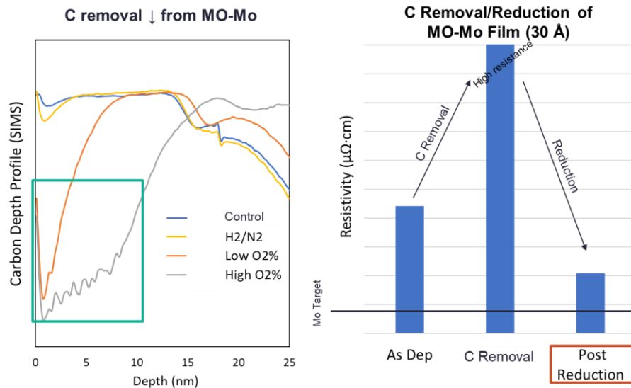
Figure 1. Complete carbon removal from MO-Mo film, but insufficient resistivity reduction after reduction
