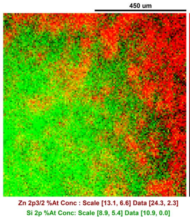
Fig1 Overlay of Zn 2p and Si 2p Atomic Concentration
