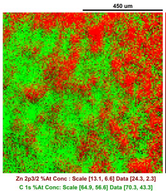
Fig2 Overlay of Zn 2p and C 1s Atomic Concentration
