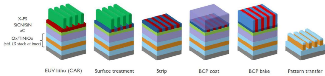
Figure 1 Illustration of P24LS pattern rectification by DSA flow
