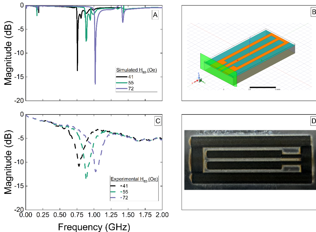
Figure 1: (A/C) simulated/measured resonance versus frequency using different magnetic field bias ( H_{ex} ), (B/D) modeled/fabricated resonator on GGG/YIG/Al.
