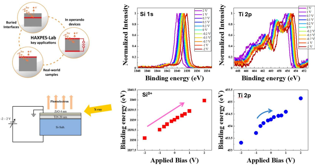
Figure 1. Key applications of HAXPES along with a Bias Applied Operando HAXPES measurement giving insight into the band alignment of a semiconductor device.
