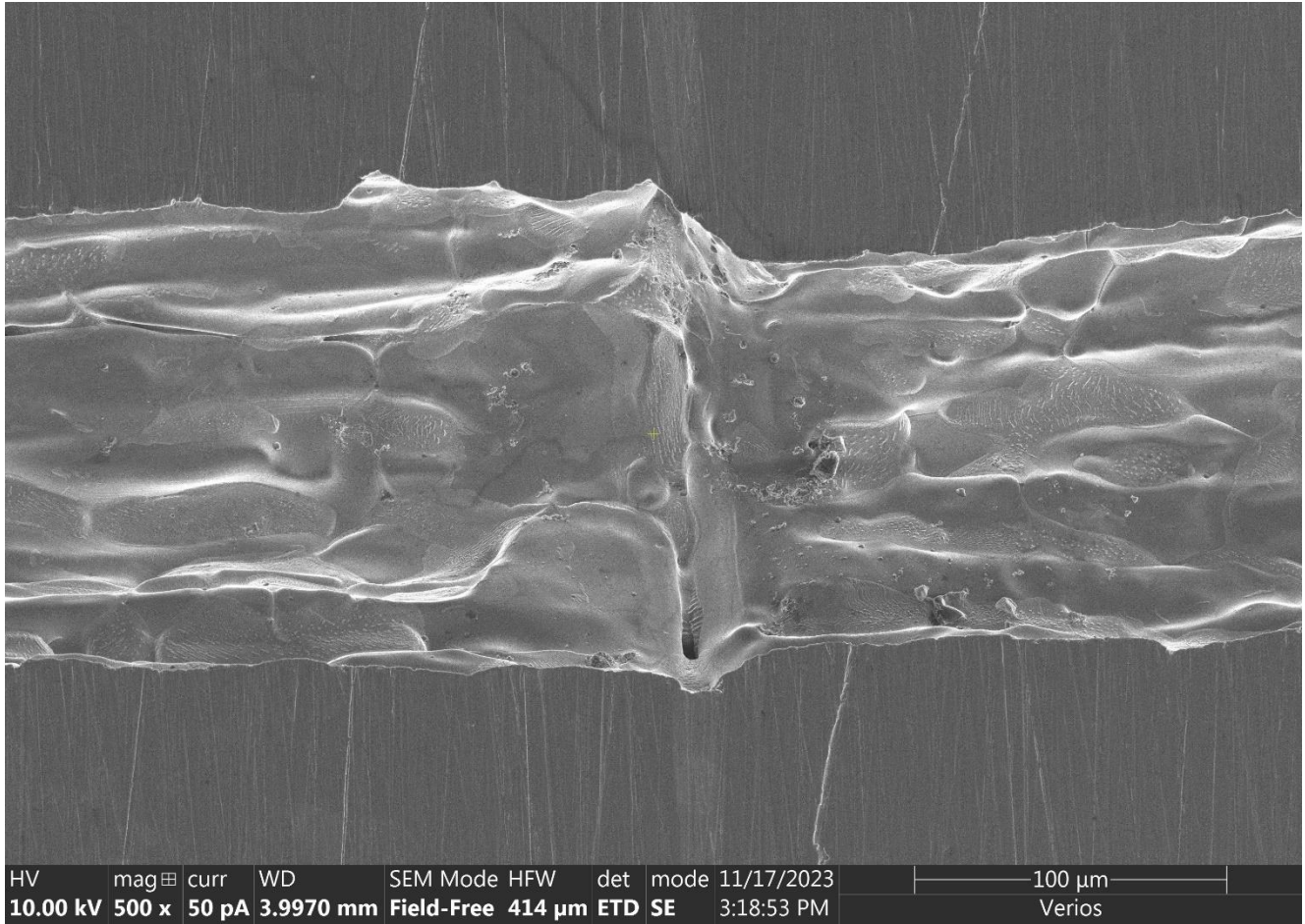
Fig 1: Scanning electron cross-section of a bronze-brazed interface between 125 \mu m and 100 \mu m inner diameter stainless steel capillaries.
