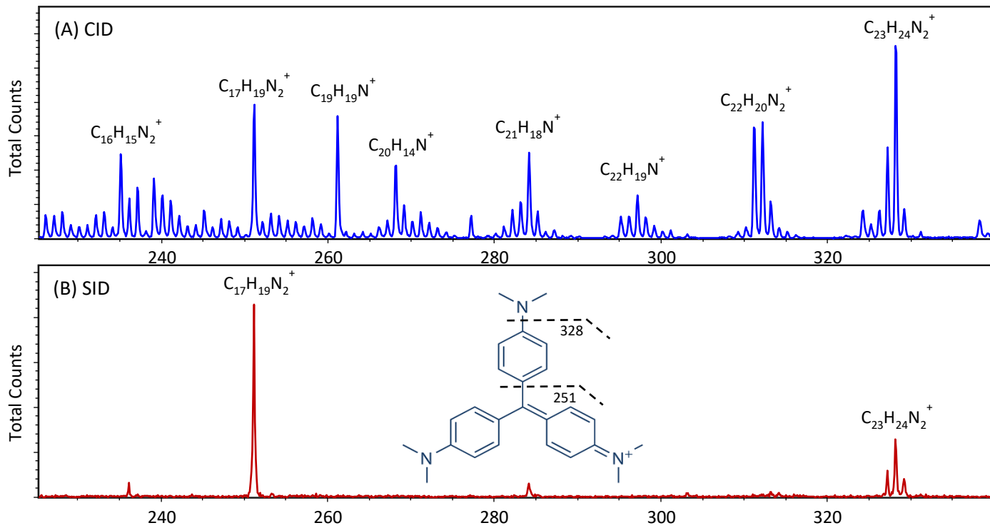
Figure 1 - CID and SID spectra of crystal violet.
