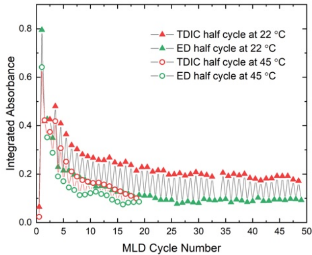
Figure 2: Integrated absorbance of amide II/I modes throughout MLD at room temperature and 45 °C, with reference spectrum collected prior to each half cycle.
