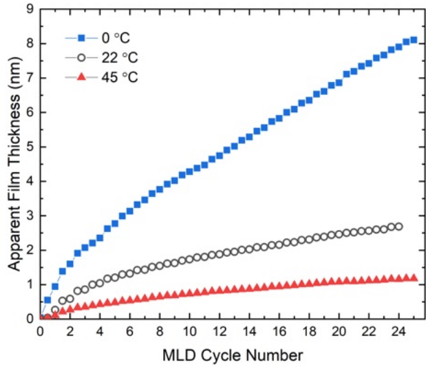
Figure 1: Thickness of TDIC/ED MLD films deposited at 0 °C, room temperature, and 25 °C, measured by in situ ellipsometry.
