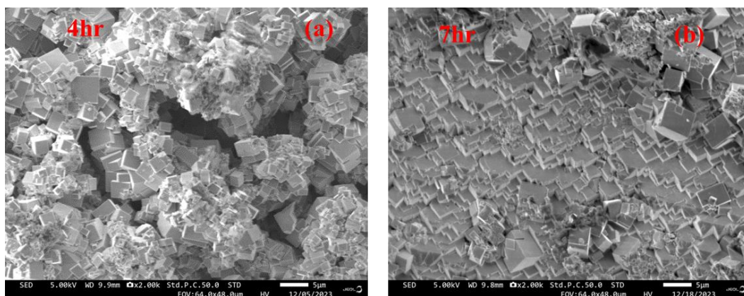
Figure1. SEM image of \text{KNbO}_3 film synthesis on \text{LiNbO}_3 substrate. (a) 4hr, (b) 7hr.
