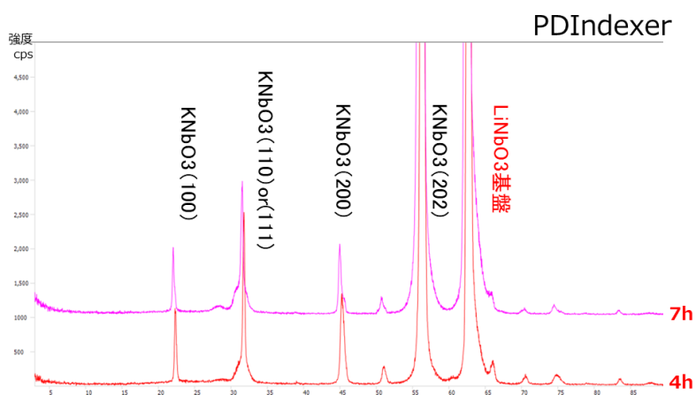
Figure2. XRD spectra of 4hr and 7hr chemical reaction time.
