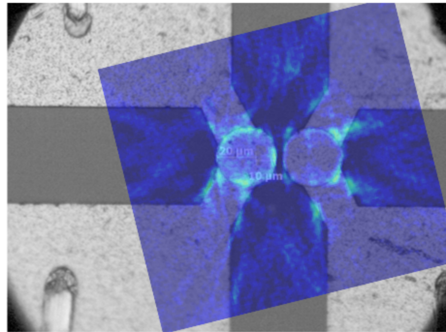
Fig 1) Left: Optical microscope image of the analysed junction. Moving to the right of the figure: The reconstructed intensity image of the HEXRR-tomo obtained by combining different HEXRR images and different positions on the sample. Lower angles reveal the morphological imperfections at the junction borders.
