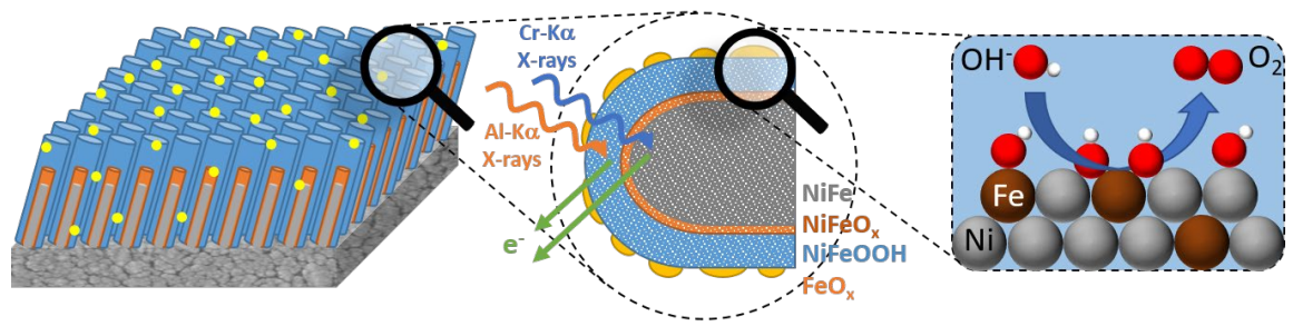
Fig. 1. Schematic representation of the investigated NiFe electrode (left), electronic structure of NiFe investigated by XPS/HAXPES (center) and Oxygen Evolution Reaction taking place at the interface between electrode and electrolyte (right).
