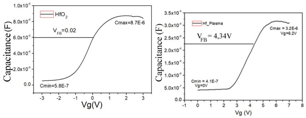
Fig. 1. C×V measurements of HfO 2 /Si (left) and HfO 2 /SiC (right).
