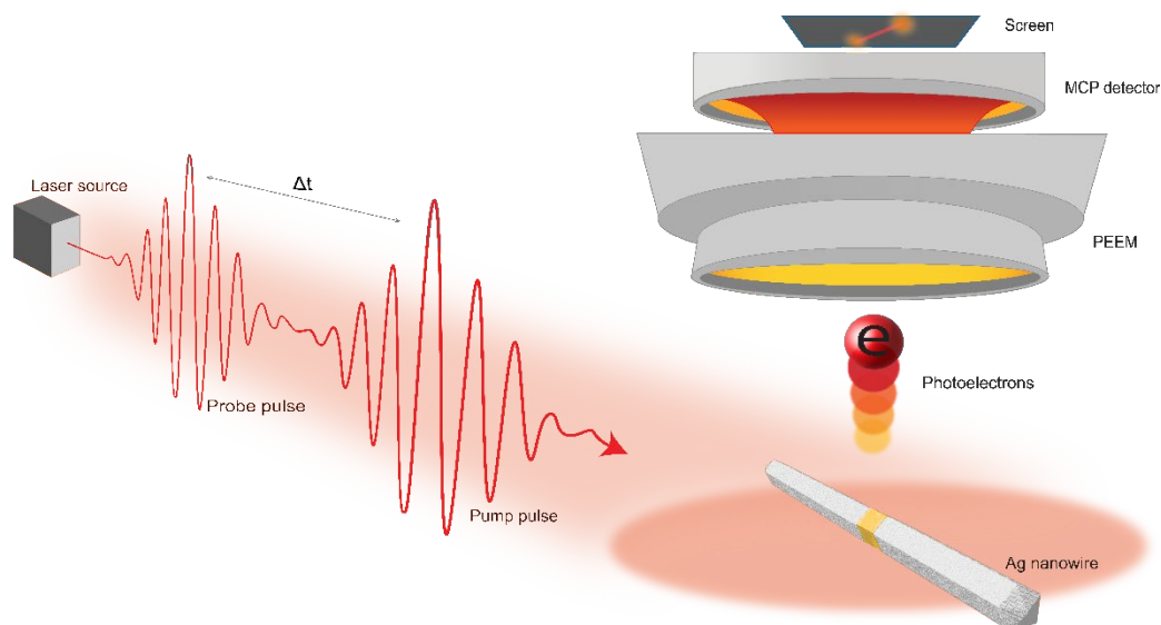
Fig 1: Schematic representation of TR-PEEM experiment on Ag nanowires.
