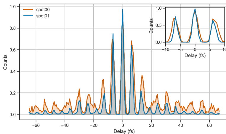
Fig 3: Example of nanowire interferometric time traces of the ends of a nanowire.
