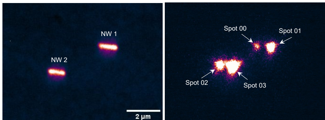
Fig 2: PEEM image of two silver nanowires using a continuous ultraviolet source and corresponding PEEM image of the same nanowires excited by short-wave infrared pulses indicating strong field enhancement at the ends of the nanowires.
