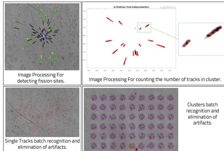
Figure 3. Automated FT Recognition for Synthetic Data
