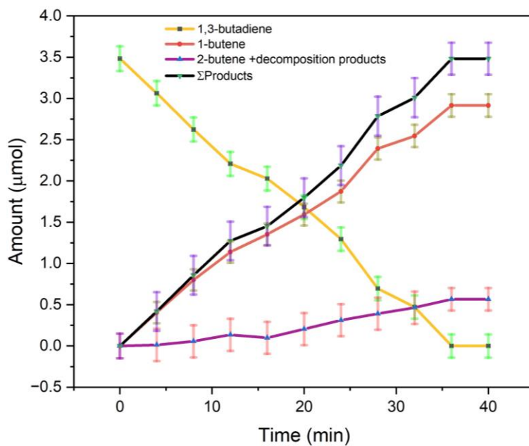
Figure: (a) Gas phase RAIR spectra of 0.10 Torr of 1,3-butadiene and 10.00 Torr of H 2 on 2.7% Pd/Cu (111) at 380 K over time. (b) Relative quantities of reactants and products during the reaction.
