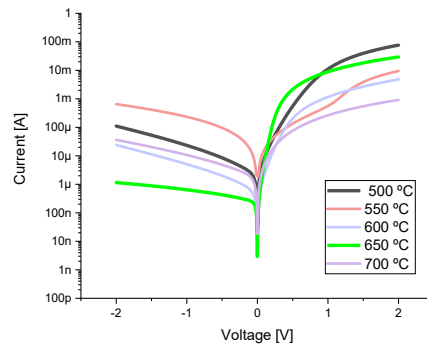
Fig. 2 – IxV semilog graph of curves under bias and reverse bias.
