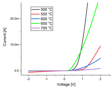
Fig. 1 – IxV curves of different annealing process.
