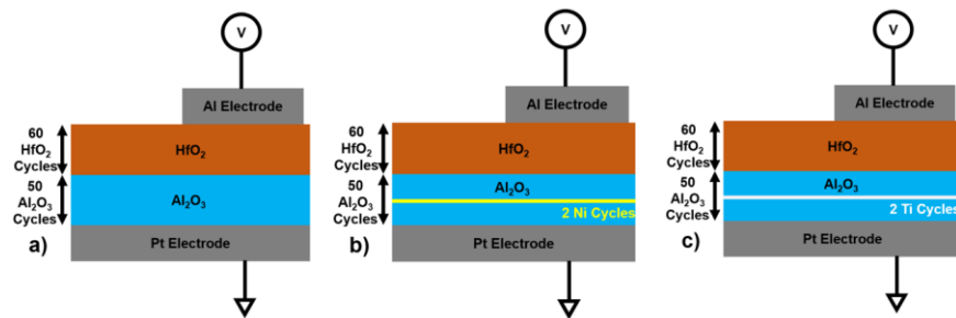
Fig. 1. Schematic cross sections of MIIM devices illustrating (a) the undoped control devices, and placement of Ni and Ti impurity layers in the (b) Ni doped device and (c) Ti doped device.
