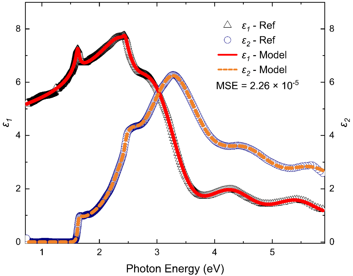
Fig 1. Dielectric function comparison between MAPbI 3 from Ghimire et al. (open symbols) and the fit produced by the parametric model (lines). The parametric model developed in this work is shown to very accurately model the experimental ellipsometric data.
