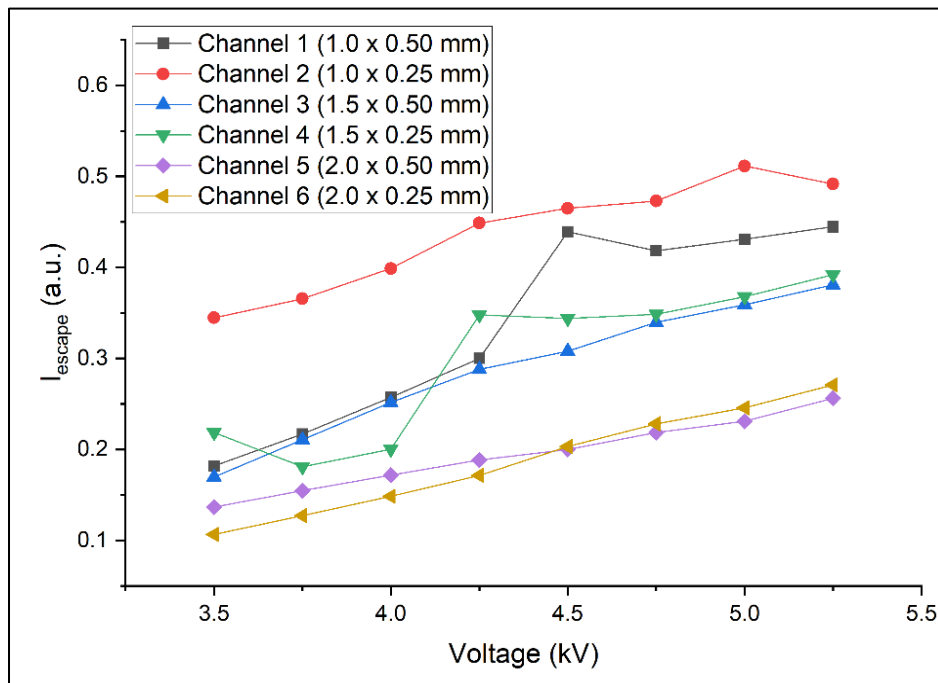
Figure 2: The fraction of total SIW light intensity that escapes the channel as functions of driving voltage and channel geometry.
