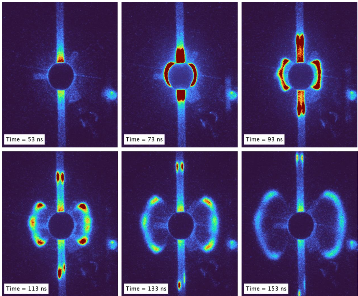
Figure 1: Plasma surface ionization wave propagating along and outside of a single channel. The dark disk in the center is a blocking plate to avoid ICCD sensor saturation.
