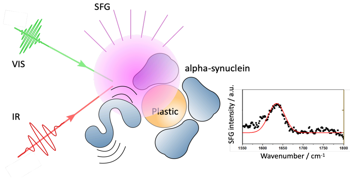
Fig 1. Schematic of the SFS experiments to follow the binding of aS to polymer particles. The SFS spectrum was recorded for aS binding the surface of polystyrene nanoparticles.
