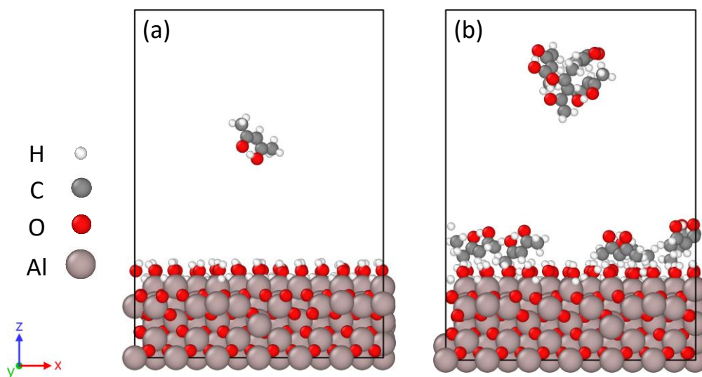
Figure. The snapshots of the front view at (a) the initial system showing the first Hacac in the gas phase and (b) the final system showing physisorbed Hacac inhibitor molecules on the surface and condensed Hacac in the gas phase.
