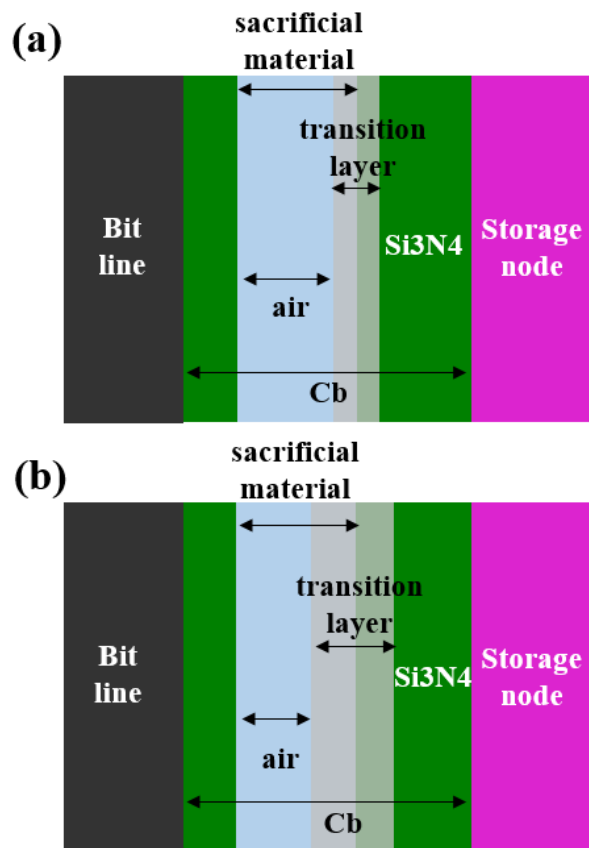
Figure 1. (a) novel air spacer structure, (b) reference air spacer structure
