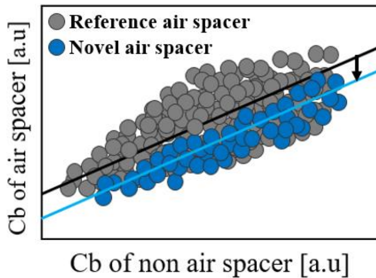
Figure 2. Electrical test measurement results for the reference and novel air spacer ; Cb of non-air spacer vs Cb of air spacer
