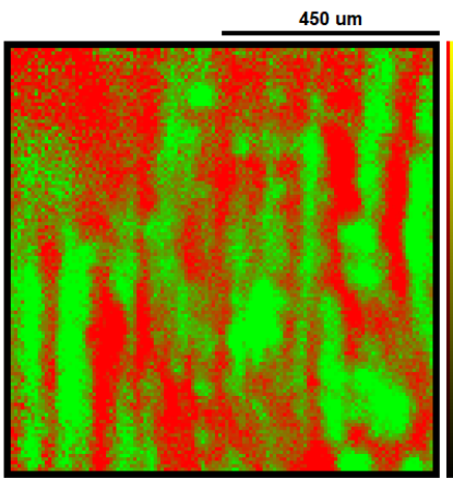
Figure 1. Overlay of Ti 2p and Sn 3d atomic concentration. The concentration of Titanium in green is between 1.7 and 2.4 percent and the atomic concentration of Tin in red is between 5.0 and 9.3 percent.
