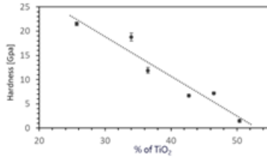
Figure 1: Hardness (nanoindentation) vs. % of TiO 2 (High resolution XPS)
