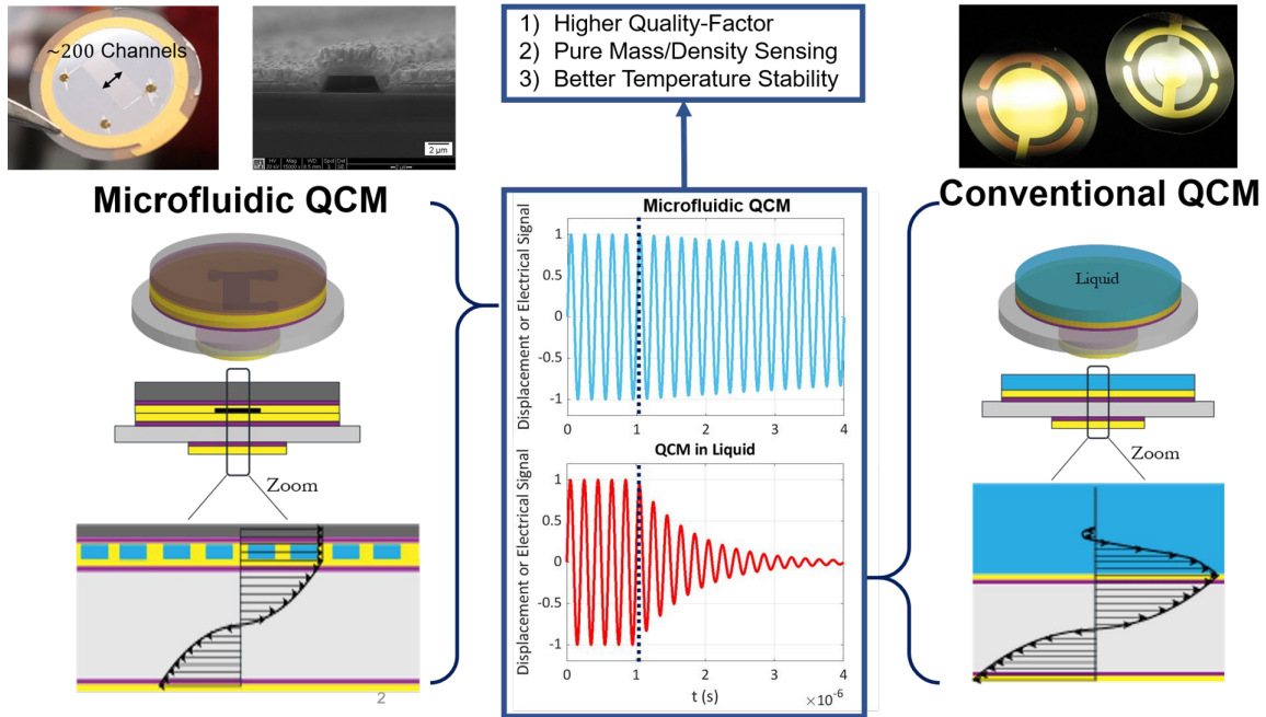
Figure 1. General schematic showing (left) the proposed microfluidic-QCM (thickness-shear mode resonators) with integrated microfluidic channels, compared to (right) conventional QCM. By largely reducing viscous damping effects, the microfluidic-QCM provides a new paradigm for biosensing.
