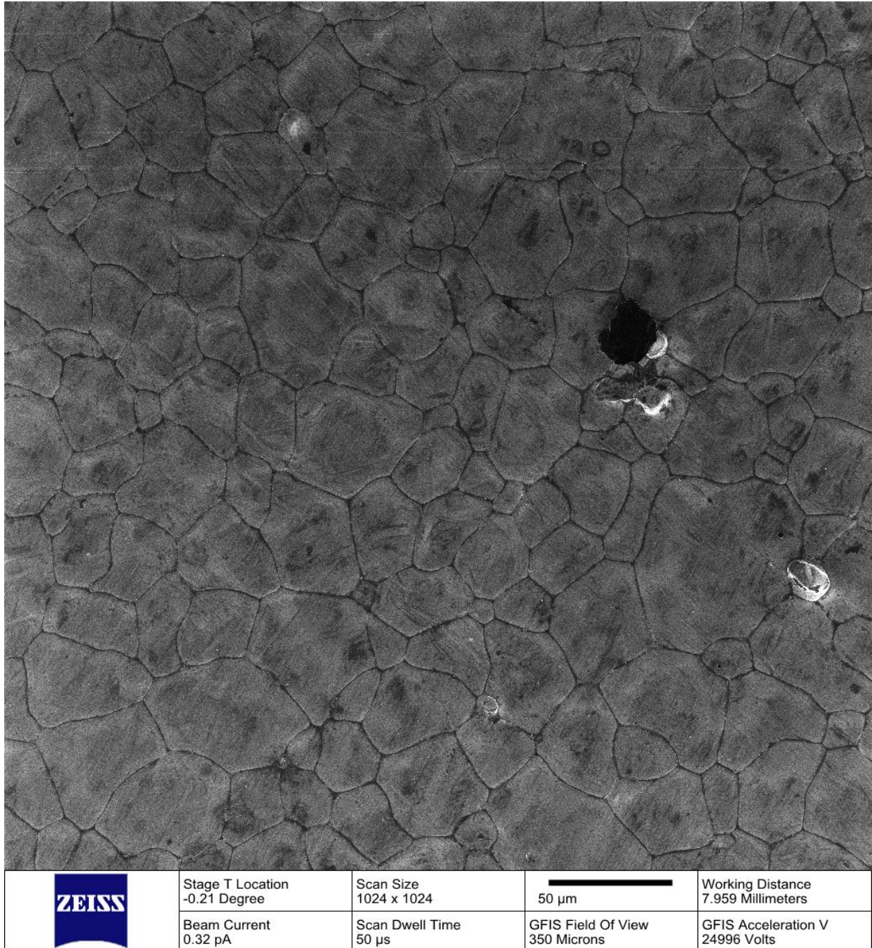
Figure. 1. HIM image of \text{BiScO}_3\text{-PbTiO}_3 ceramic showing large grain size, no porosity and flat, uniform topography correlated with good piezoelectric properties.
