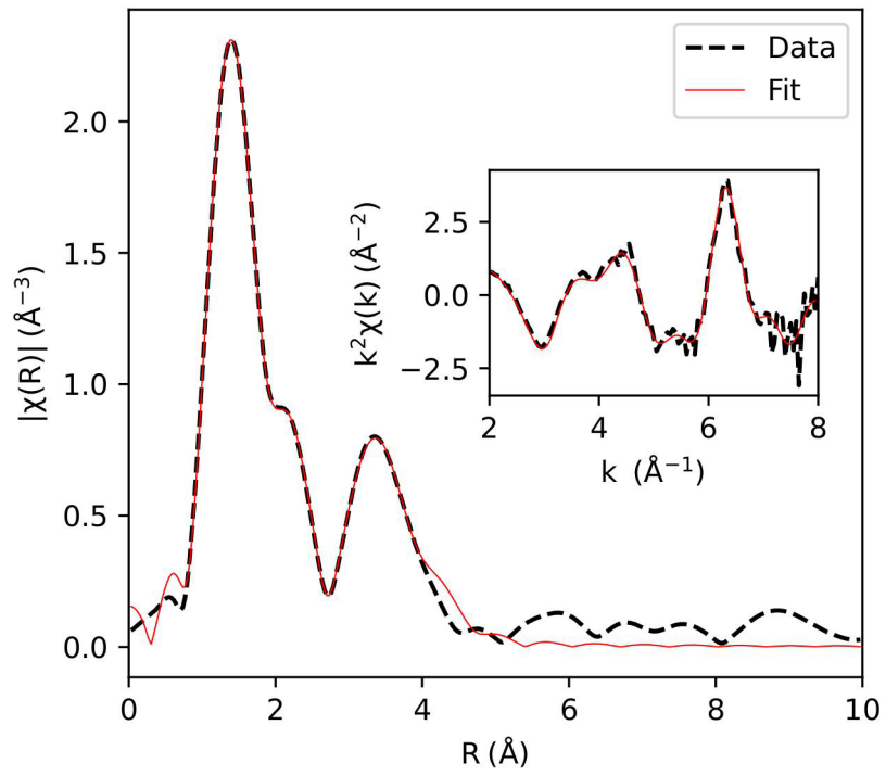
Sample #2 EXAFS spectrum with fit in both r-space and k-space on the inset plot
