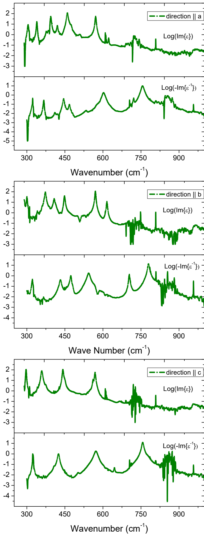
Figure 1: The imaginary part and the imaginary part of its inverse of the dielectric tensor function for \text{LiGaO}_2 derived from the point-by-point fit to experimental Mueller matrix data for the mid-infrared spectral range. The dielectric tensor components in directions parallel to a, b, and c are shown. Please note the logarithmic scales.
