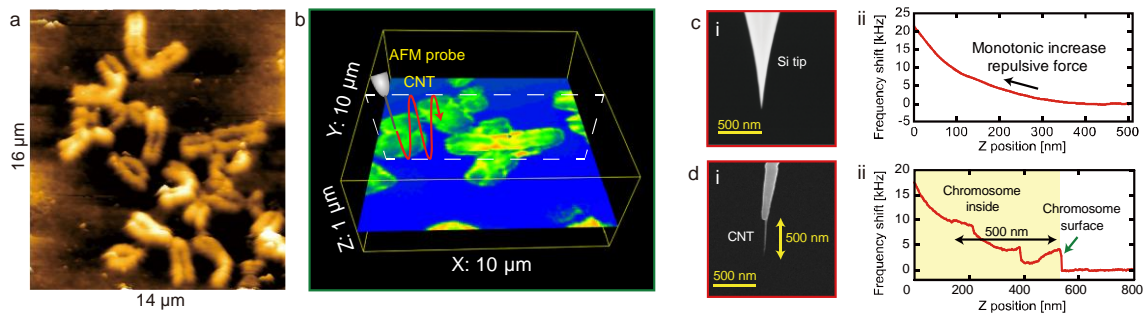
Fig. 1: (a) 2D- and (b) 3D-AFM images of human chromosome. (c-d) (i) SEM images of tips and (ii) \Delta f curves on human chromosome using (c) conventional tip and (d) CNT tip.
