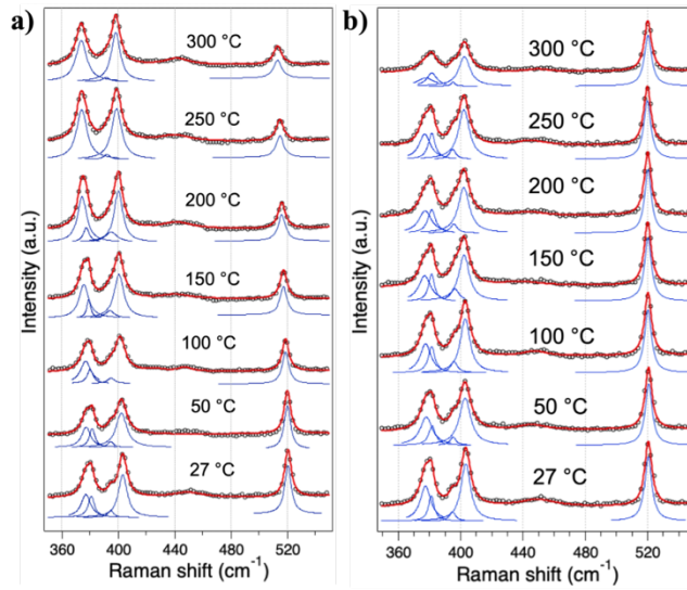
Figure 1: Temperature-dependent Raman spectra of MoS 2 on Au acquired at a) temperature and b) room temperature post-anneal. E 2g and A 1g peaks occur at ~ 383 cm -1 and 407 cm -1 , respectively.
