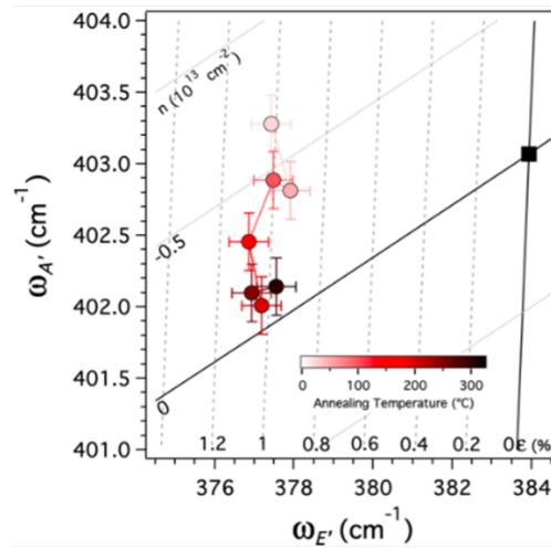
Figure 2: Temperature-dependent strain and doping of SL-MoS 2 on Au after annealing at progressively higher temperatures.
