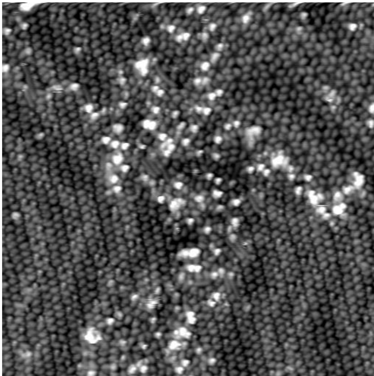
Figure 1. STM images of proline on Au(111). The images shows two configurations: a pentamer formation (top right), and a dimer or catamer formation (bottom left).
