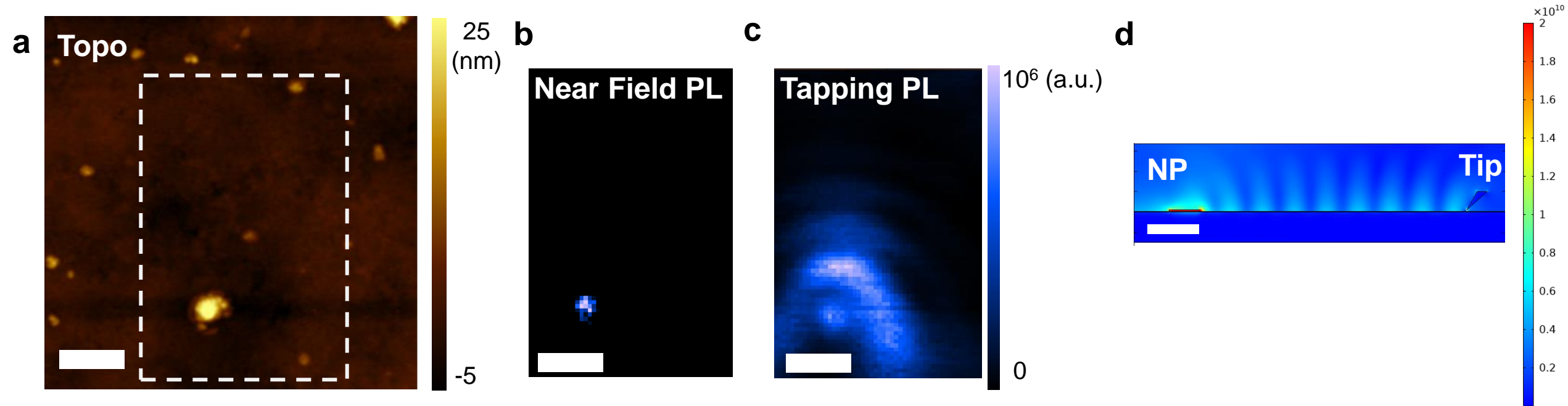
(a) Topography of Al 2 O 3 / CdSe-CdS quantum nanoplatelets (NP) on Au. (b) Near-field (Contact PL – tapping PL) and (c) tapping mode tip-enhanced photoluminescence map at NP emission wavelength. (d) Finite element electromagnetic wave simulation of Al 2 O 3 /NP/Au with plasmonic Au tip. Scale bars indicate 500 nm.
