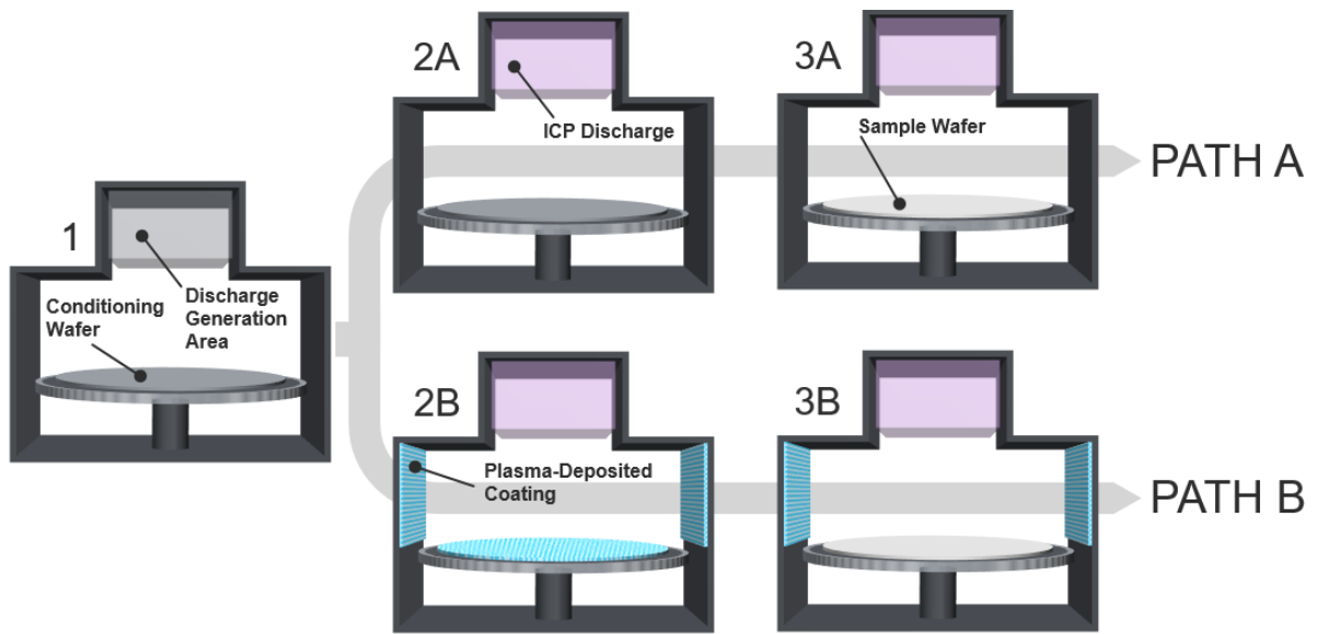
Figure 1: Comparison of PATH A, etching pathway without coating, to PATH B, etching pathway with coating
