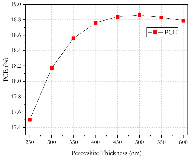
Figure 3. Absorber layer thickness versus PCE.
