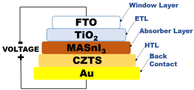
Figure 1. The n-i-p perovskite solar cell structure.
