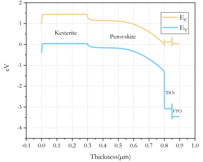
Figure 2. The band diagram of the n-i-p PSC at equilibrium.
