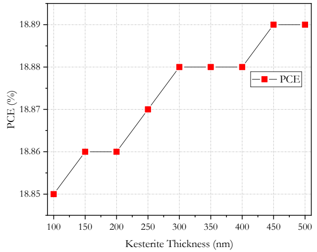
Figure 4. Kesterite layer thickness versus PCE.
