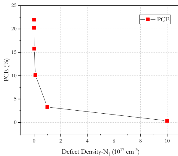
Figure 5. Absorber layer defects N_t versus PCE.
