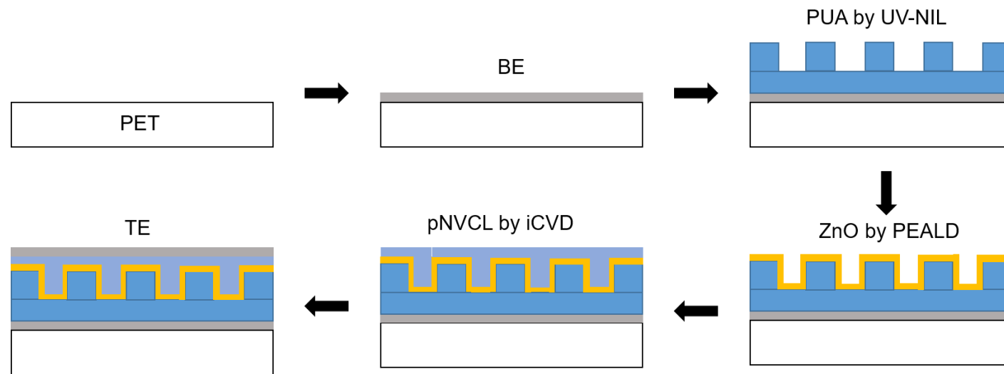
Figure 1: fabrication steps of multi-stimuli responsive core-shell nanorods.
