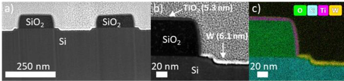
Figure 1 Cross-sectional TEM images for TiO 2 /W orthogonal selective deposition on SiO 2 /Si trench-shaped patterned substrate (200 nm half-pitch): a) broad view of patterns, b) magnified view of one pattern, c) EDX of image in b).
