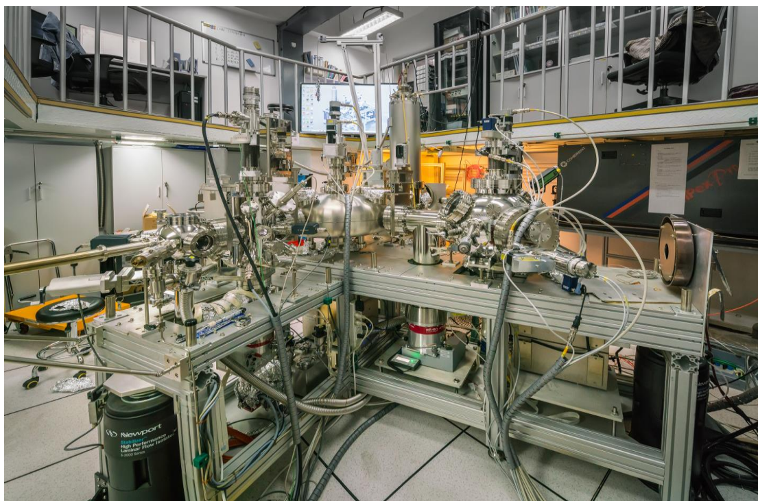
Fig. 3 Photo of the home-made Combi-LMBE-SPM system
