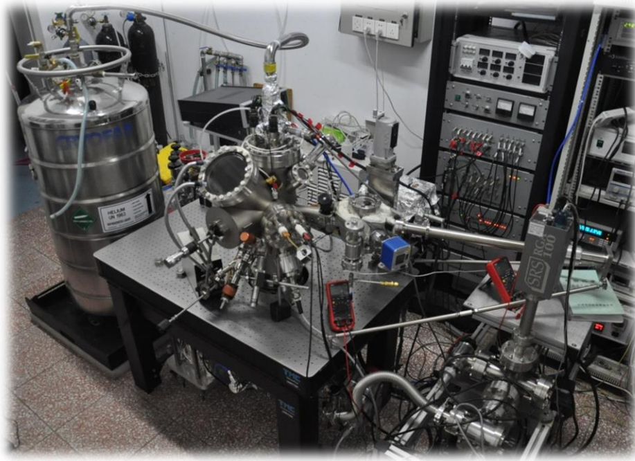
Fig. 1 Photo of the home-made UHV-VT-STM system
