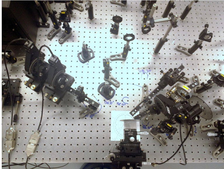
Fig. 1. Photograph of the sample environment of Time-resolved Ellipsometry setup
