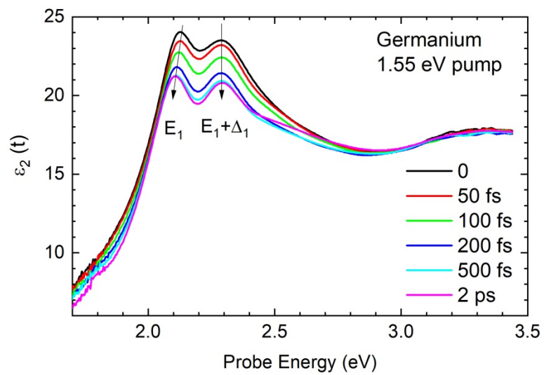
Fig. 2. Dynamics of the imaginary part of the dielectric function of Ge
