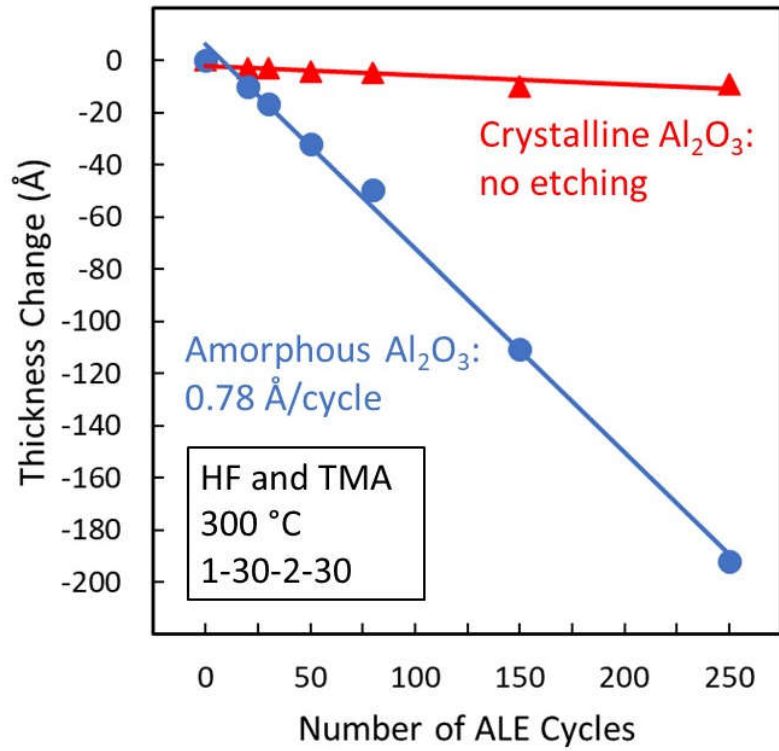
Supplemental Figure 1. ALE for amorphous (blue) and polycrystalline (red) Al 2 O 3 using HF and TMA at 300 °C.
