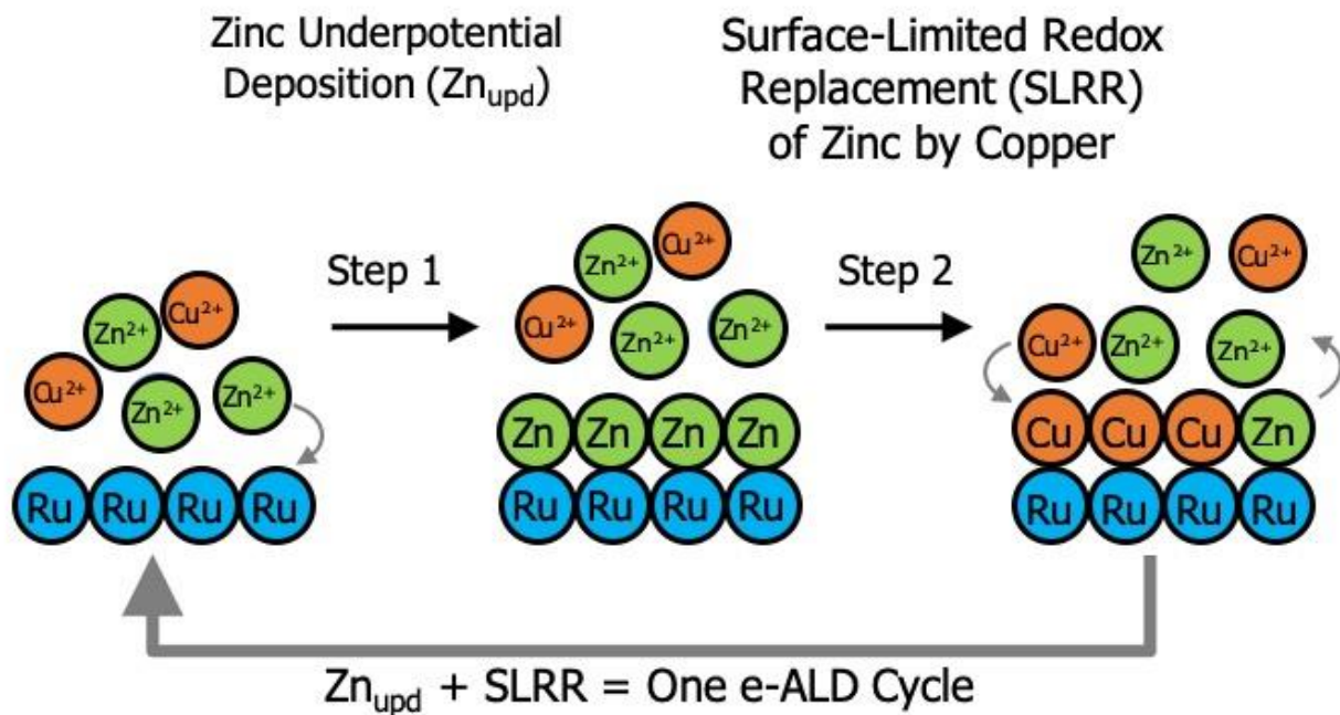
Figure 1. Schematic representation of the Cu electrochemical atomic layer deposition process.
