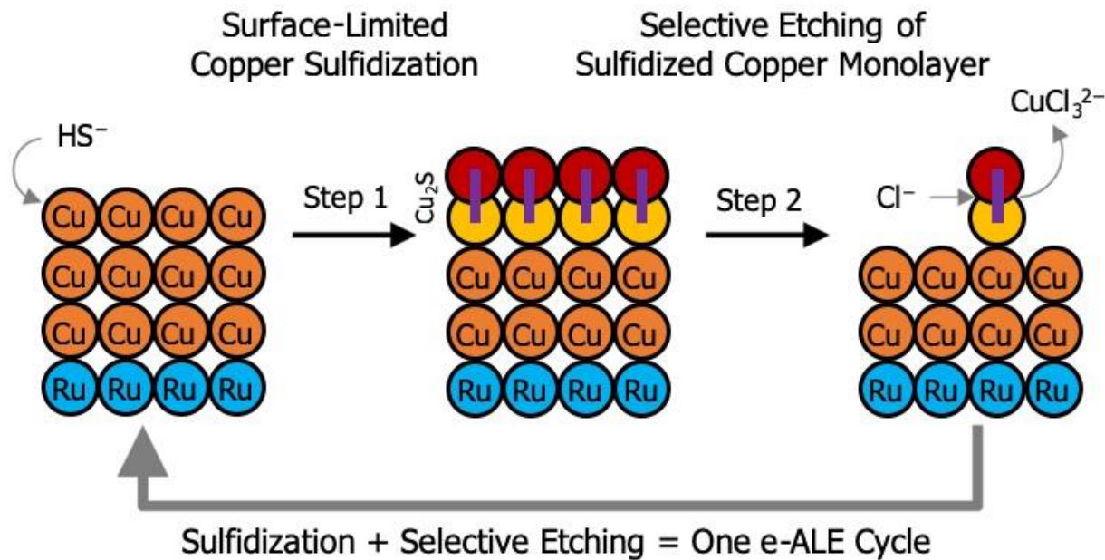
Figure 2. Schematic representation of the Cu electrochemical atomic layer etching process.
