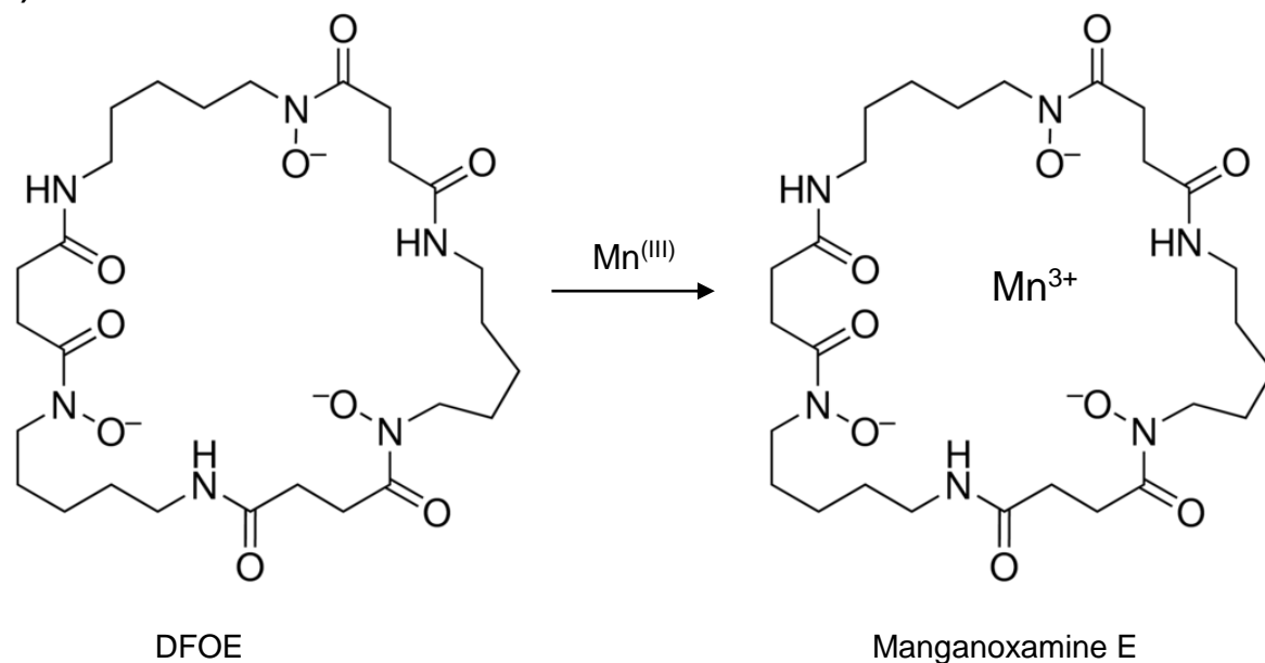
Figure 1. (A) Manganese complexation with DFOB to form manganoxamine B, similar complexation occurs with Fe(III) to form ferrioxamine B (FOB). (B) Complexation with DFOE.
