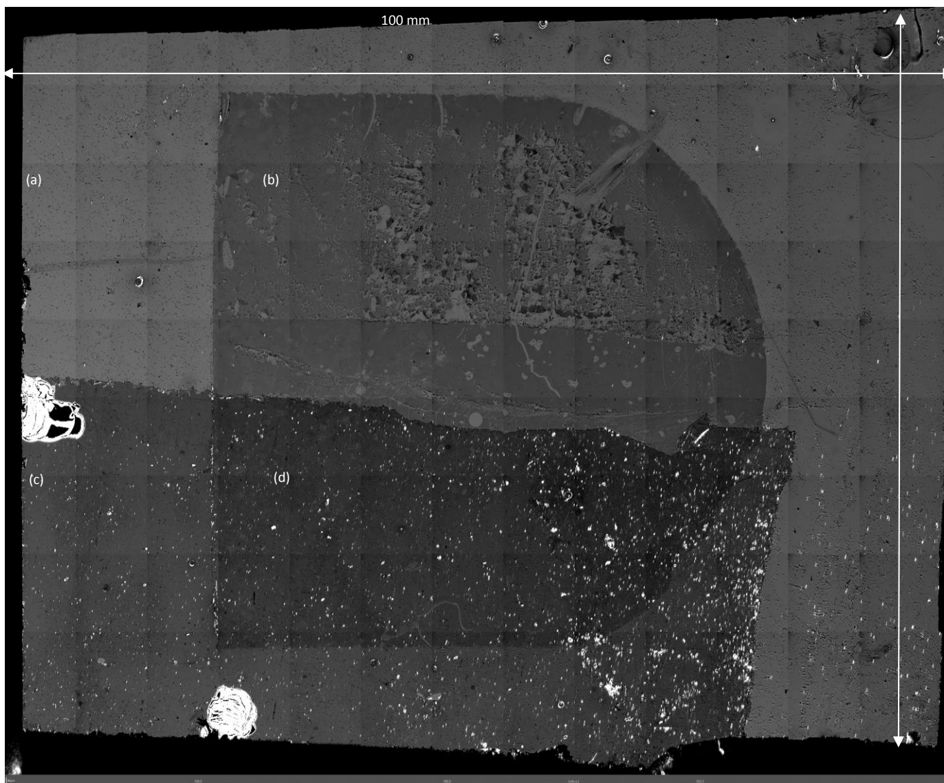
Figure 1 hBN and Graphene monolayer on Si/SiO 2 substrate. Visualized in less than 6 minutes. (a) substrate only, (b) hBN only, (c) Graphene only and (d) monolayer graphene on monolayer hBN.
